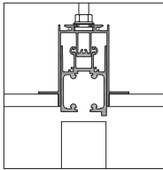
incassato, binario sporgenza minima mm 10, filo porta - 15 built-in, track minimum protrusion downwards 1/2", flush to door - 1/2"
