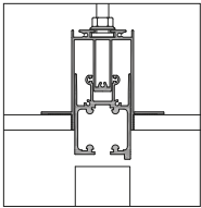
incassato, per allineamento con armadi e boiserie Surface, filo porta - 30 built-in, for alignment with wardrobes and Surface wall panelling, flush to door - 1 1/4"
