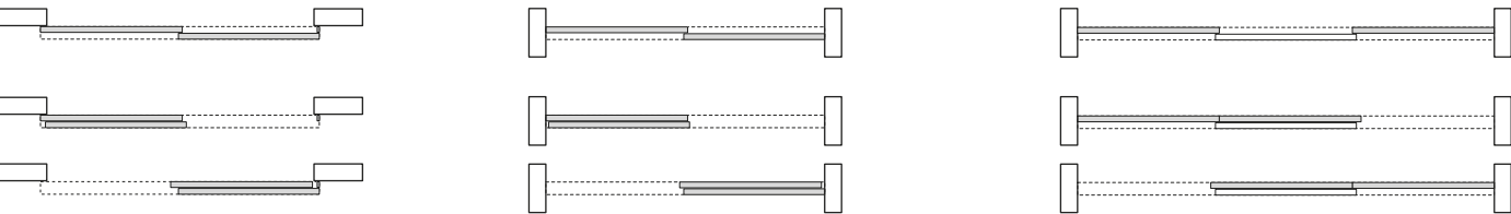
ante apribili alternate alternate opening doors ante apribili alternate alternate opening doors ante apribili alternate alternate opening doors
