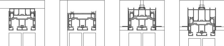
soffitto ceiling parete wall incassato a filo flush built-in incassato, per allineamento con armadi e boiserie Surface, filo porta - 30 built-in, for alignment with wardrobes and Surface wall panelling, flush to door - 1 1/4"
